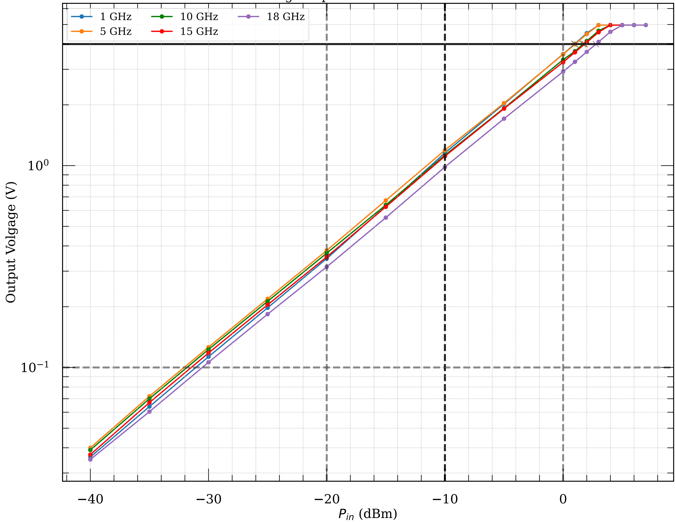
Measured voltage-to-power curve of detector module057
